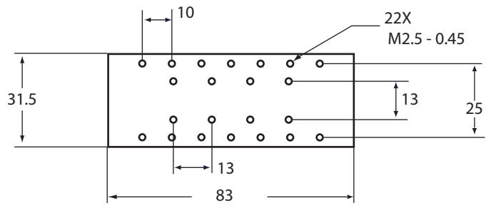
Top View (50 mm Carrier)
